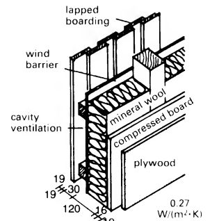
⑬ Timber frame (insulation between the posts) 0.27 W/(m 2 ·K)
